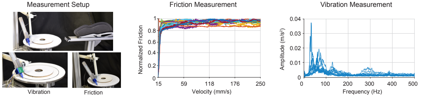
Fig. 2. Measurements and perceptual user study setup. Turntable on which a mechanical arm is used to capture friction and vibration of drawing tools. There is a holder for a human arm (during user studies) to provide consistent grip and orientation. In the middle, we can see normalized friction measurements recovered using our setup. On the right is the accelerometer response for a fixed velocity.
