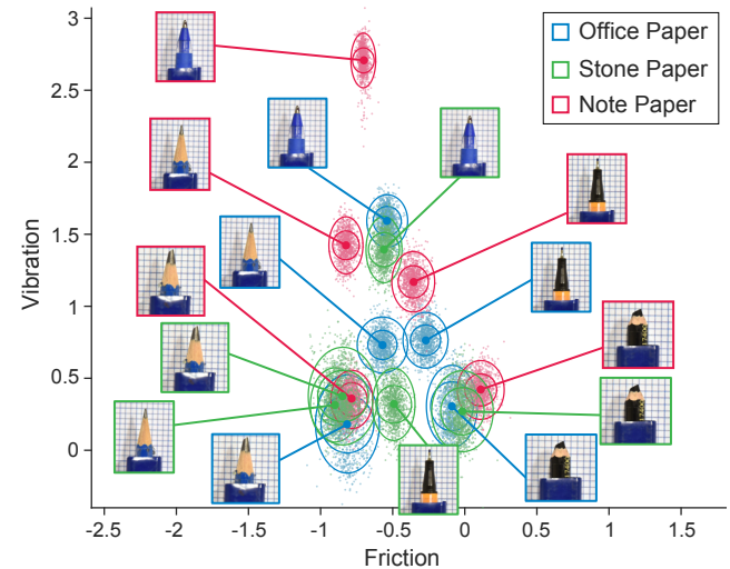
Fig. 9. The perceptual space obtained using our data and optimization. The axis are correlated with vibration and friction measurements. Confidence intervals obtained by bootstrapping visualize 95% and 68% regions.
